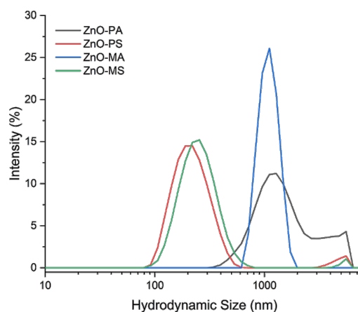
Figure 3: Hydrodynamic size distributions of the synthesized ZnO nanoparticles determined by DLS.
