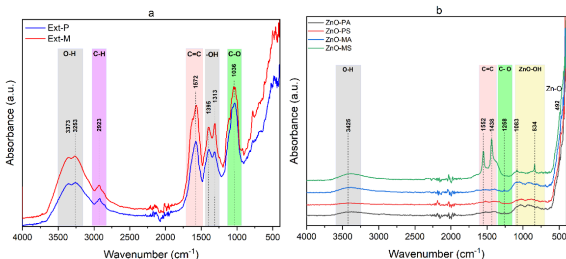
Figure 1: FTIR spectra of (a) the lyophilized aqueous extracts of P. auritum (Ext-P) and M. pudica (Ext-M) and (b) the corresponding ZnO nanoparticles after calcination at 400 °C.
