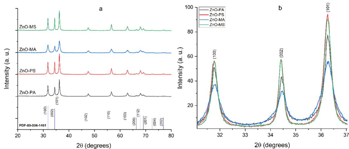
Figure 2: X-ray diffraction patterns of the synthesized ZnO nanoparticles: (a) complete diffractograms and (b) enlarged view of the (100), (002), and (101) reflections.
