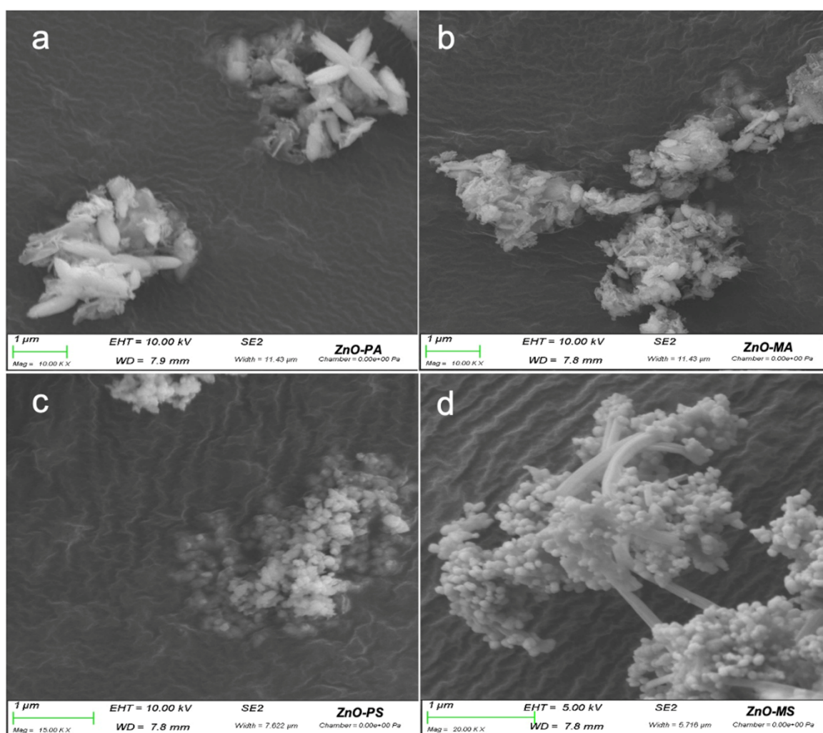
Figure 4: FESEM micrographs of the synthesized ZnO nanoparticles: (a) ZnO-PA, (b) ZnO-MA, (c) ZnO-PS, and (d) ZnO-MS.
