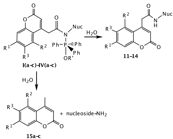
Scheme 2: Hydrolysis of proposed intermediates I(a-c)-IV(a-c)
