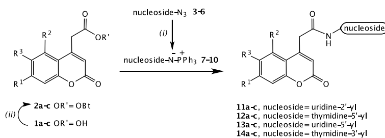
Scheme 1: Preparation of coumarin labeled nucleosides, (i) PPh 3 , acetonitrile, (ii) HOBT, DCC, dioxane
