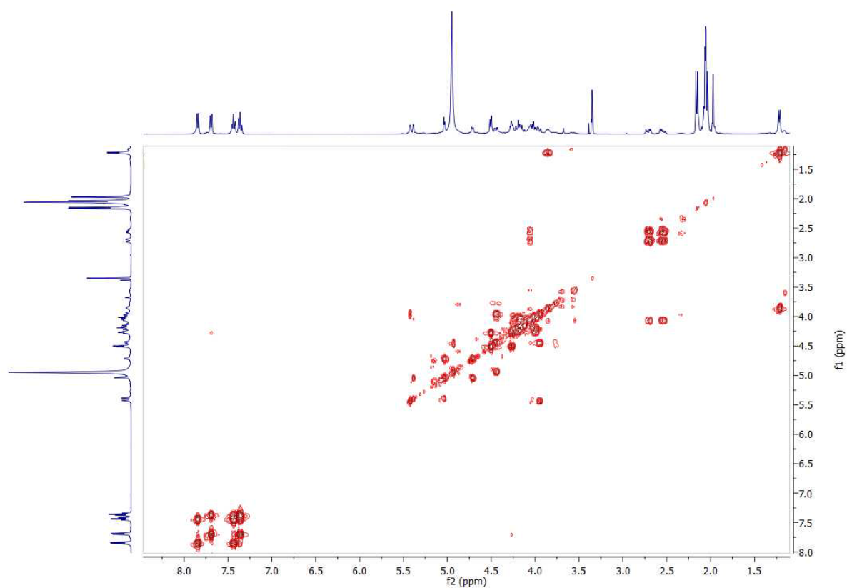
Compound 7 (400 MHz, D 2 O): 1 H, H,H-COSY
