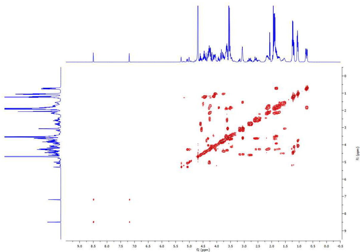
Compound 8 (400 MHz, D 2 O): 1 H, H,H-COSY
