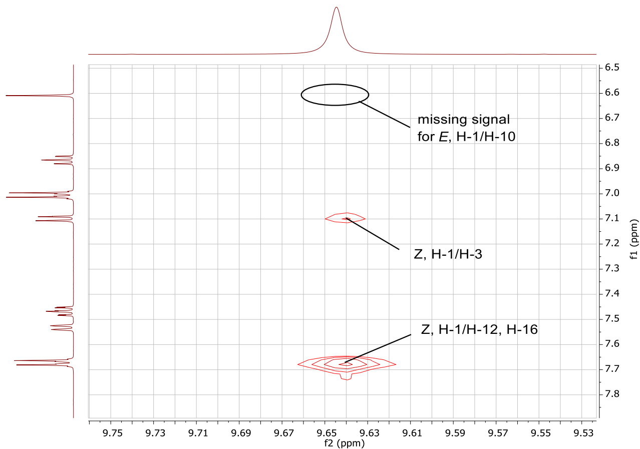
Figure S10. Section of the NOESY NMR spectrum of hemi-indigo Z-1b in DMSO- d_6 . The NOE cross-signal between protons H-1 and H-12 indicate their close proximity and, therefore, prove the Z -conformation. In the E -conformation a cross signal between protons H-1 and H-10 is expected but it is not observed.
