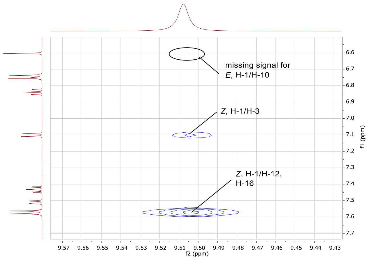
Figure S7. Section of the NOESY NMR spectrum of hemi-indigo Z-1a in DMSO- d_6 . The NOE cross-signal between protons H-1 and H-12 indicate their close proximity and, therefore, prove the Z -conformation. In the E -conformation a cross signal between protons H-1 and H-10 is expected but it is not observed.
