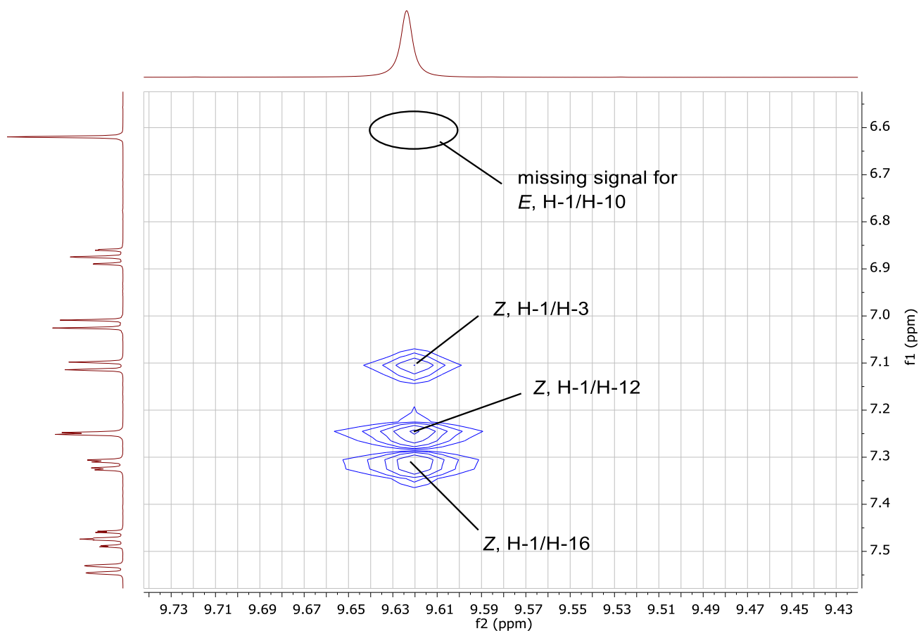
Figure S13. Section of the NOESY NMR spectrum of hemi-indigo Z-1c in DMSO- d_6 . The NOE cross-signal between protons H-1 and H-12 indicate their close proximity and, therefore, prove the Z -conformation. In the E -conformation a cross signal between protons H-1 and H-10 is expected but it is not observed.
