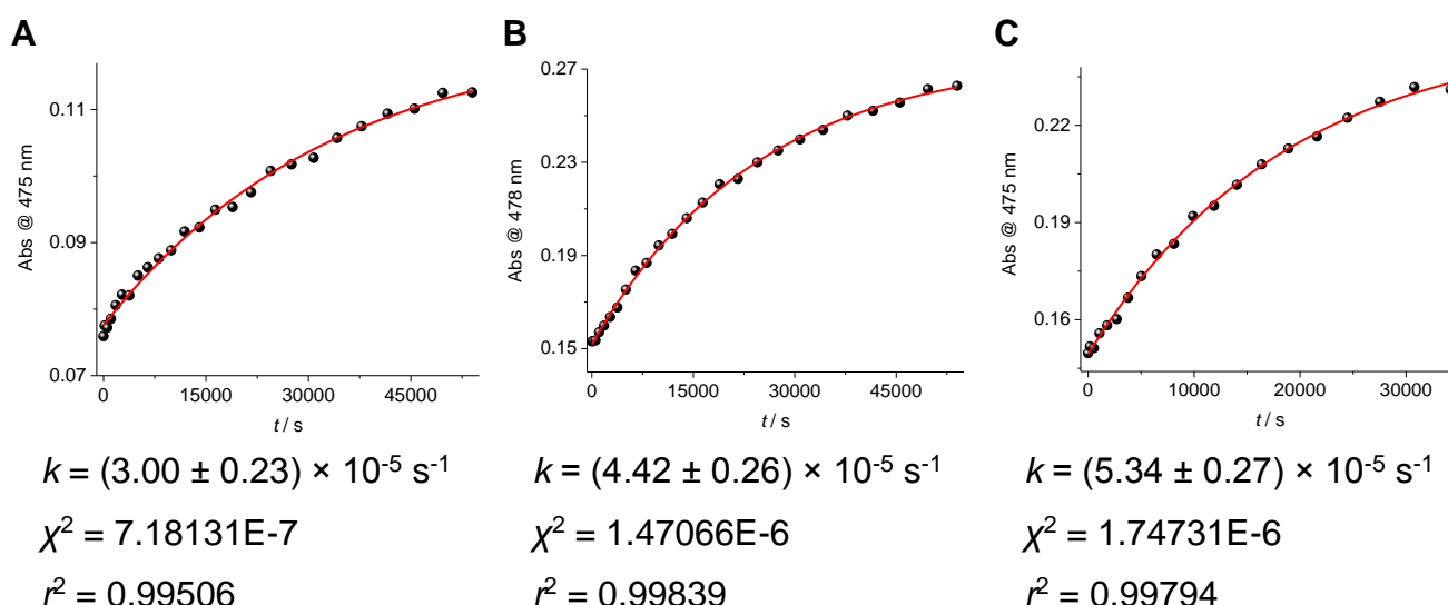
Figure S3. Evolution of the absorbance (black spheres) for the thermal E-Z isomerization in water at 60 °C of (A) 1b , c = 10 \mu\text{M} , \lambda_{\text{det}} = 475 \text{ nm} , solution contained 1% (v/v) EtOH for the solubility reasons; (B) 1c , c = 20 \mu\text{M} , \lambda_{\text{det}} = 478 \text{ nm} ; (C) 2 , c = 20 \mu\text{M} , \lambda_{\text{det}} = 475 \text{ nm} . Solid red line indicates the fit of the experimental data to the monoexponential model.
