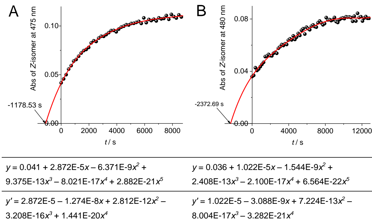
Figure S4. Quantum yield measurement of the E-Z photoisomerization of hemi-indigo derivatives (A) 1c and (B) 2 upon irradiation with 590 nm starting from the pre-irradiated mixtures of E- and Z-isomers (PSS 470 , black squares) in water, 20 °C. The whole photoconversion kinetics was fitted to the corresponding polynomials (red solid line).
