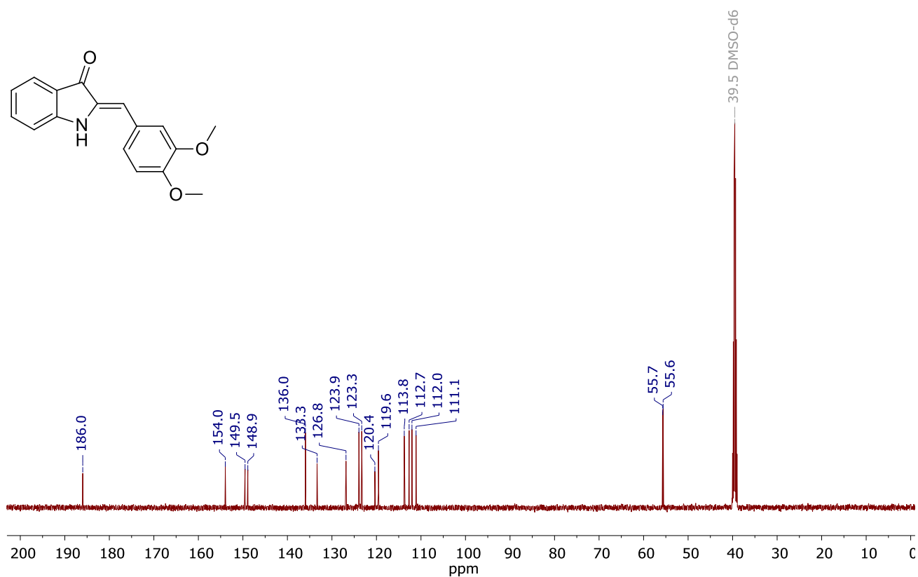
Figure S12. ^{13}\text{C} NMR spectrum of Z-1c in DMSO- d_6 .
