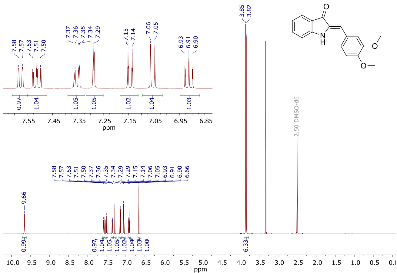
Figure S11. ^1\text{H} NMR spectrum of Z-1c in DMSO- d_6 .
