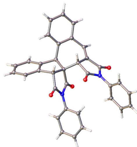
Figure S1. ORTEP representation of compound 2a (thermal ellipsoids are shown at 50% probability)
