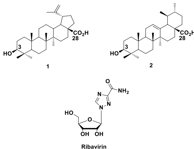
Figure 1. Structures of RBV, betulinic acid (1), and ursolic acid (2)
